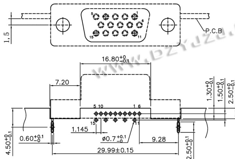
Recommended P.C.B Layout (component side)
